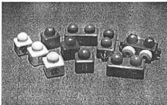
Figure 1 The complete Electronic Block family: the three sensor blocks are to the left, the four logic blocks are in the centre, and the action blocks to the right.
